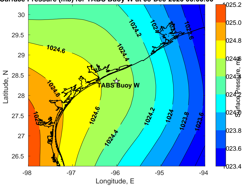
Surface Pressure (mb) for TABS Buoy W at 08-Dec-2020 06:00:00
